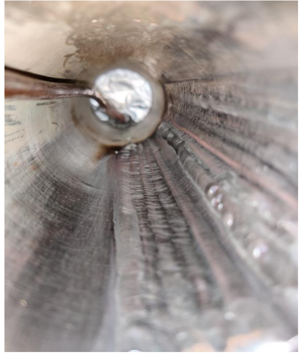
Pipe ID Overlay using GTAW Process
