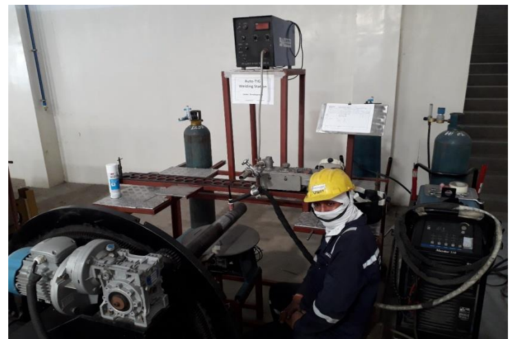
Automatic TIG Welding Station
